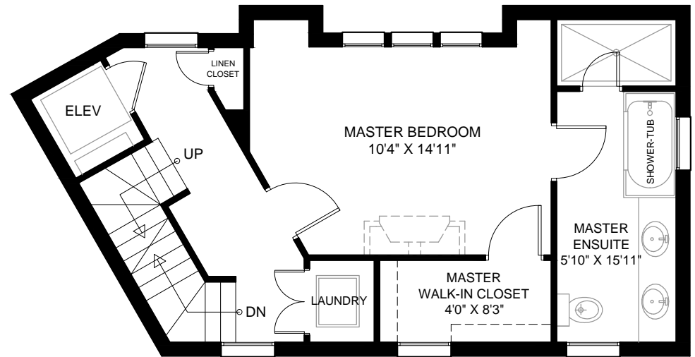
3RD FLOOR
