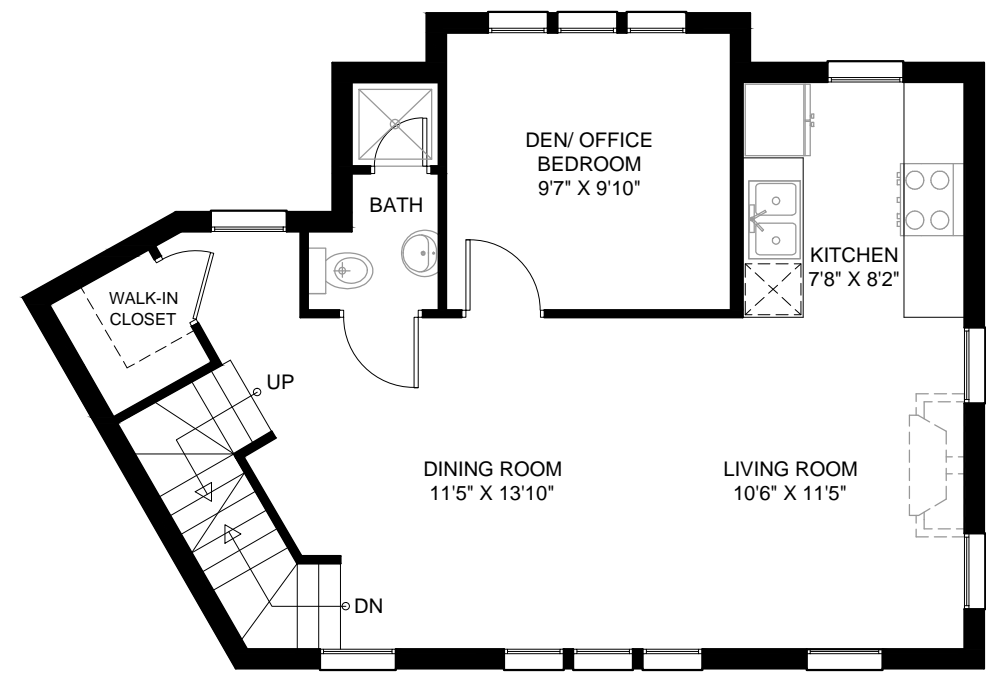
2ND FLOOR
